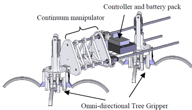
Fig. 9: Robot Treebot [9].
